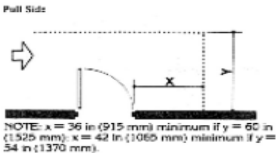
(a) Front Approaches — Swinging Doors
